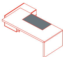
Right desk arranged for electrification, with black leather liftable desk pad and side container 1AS4821: L 242 D 135 H 75
